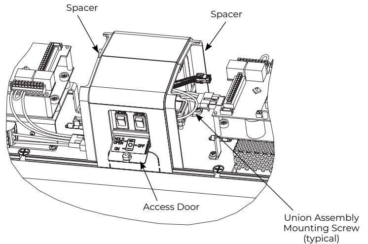
Figure 18 Union Assembly - View From Floor
